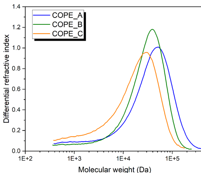
Figure 3. The molecular weight distributions of the three tested copolyester HMAs.
