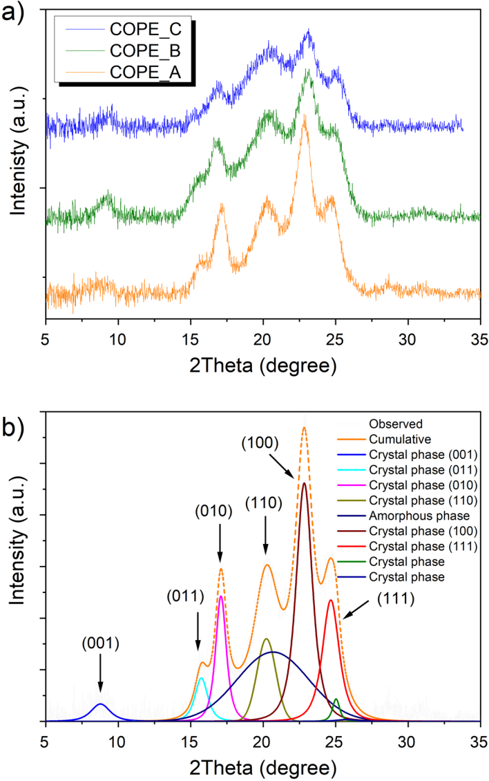
Figure 4. (a) Wide angle X-ray scattering (WAXS) spectra of analyzed samples and (b) fitting of WAXS spectra of COPE_B.
