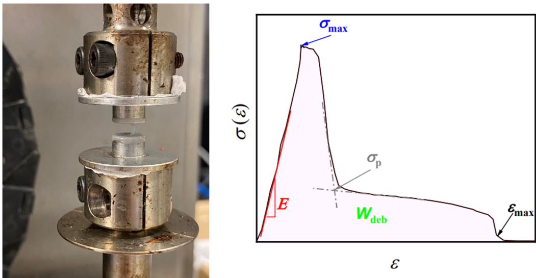
Figure 1. Schematic stress–strain curve obtained during probe-tack experiments. Reprinted with permission from reference [25] (CC BY licensed, Copyright (c) 2022).
