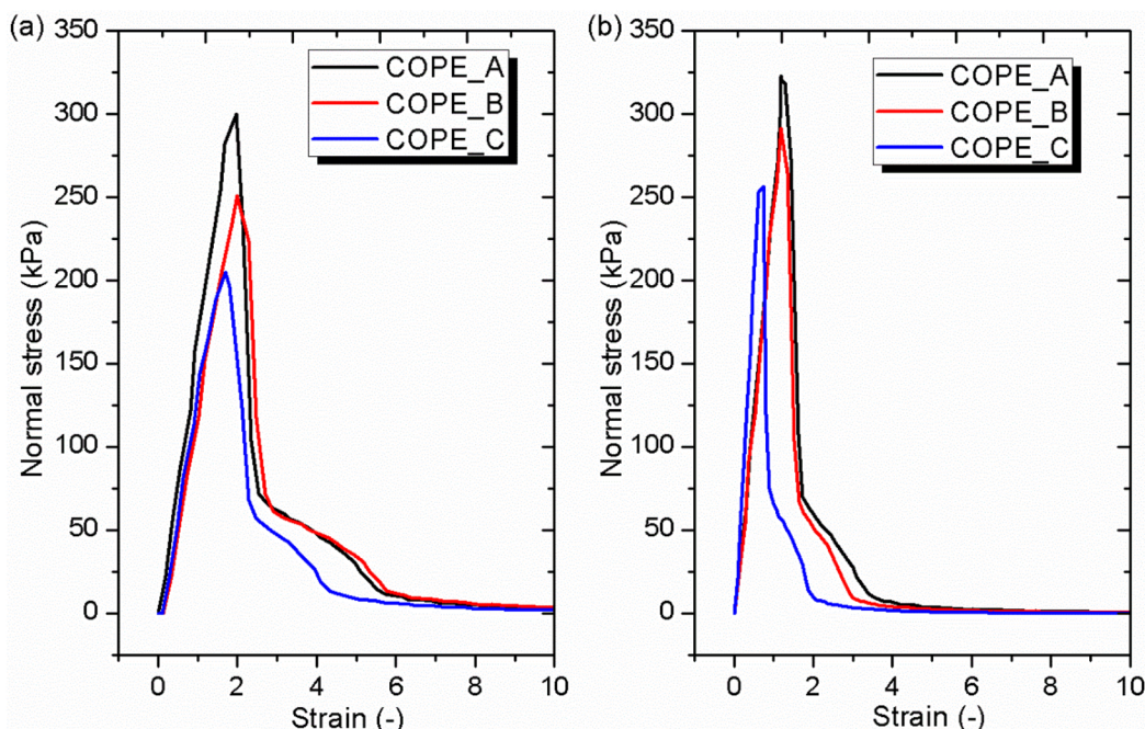
Figure 8. Stress-strain curves for tested hot melt adhesives at T = T_m + 10^\circ\text{C} (a) and at T = 180^\circ\text{C} (b). The test velocity was 0.314 mm/s.
