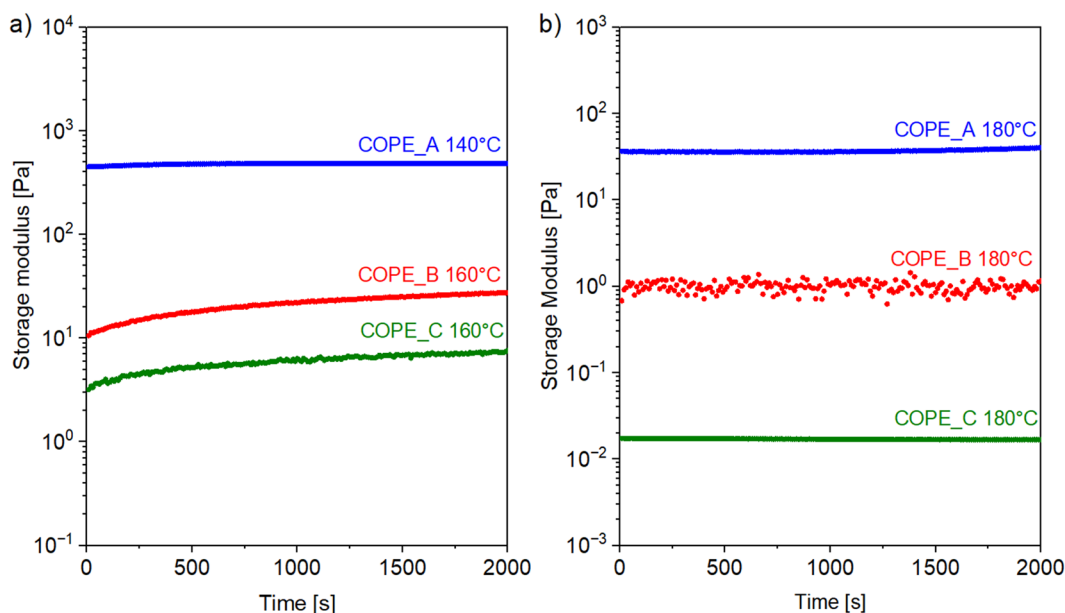
Figure 6. The changes in the storage modulus of copolyesters over the time at different temperatures.
