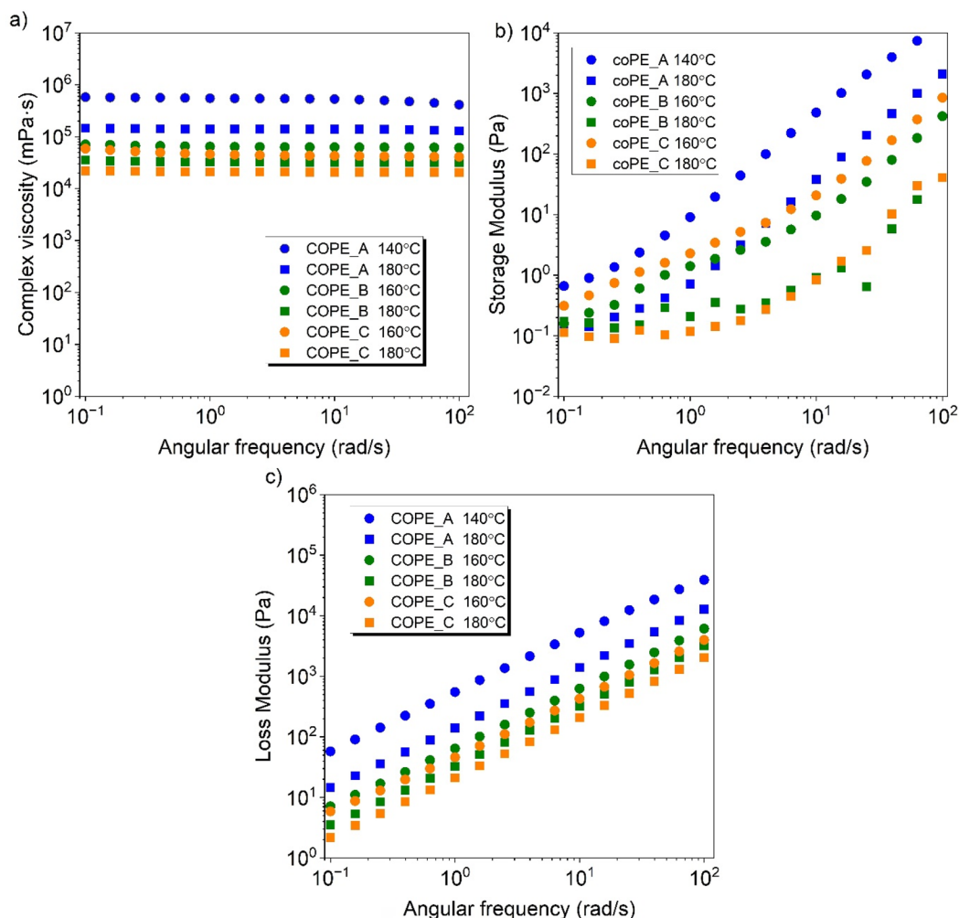
Figure 7. (a) Complex viscosity and (b) storage modulus of the copolyesters (c) loss modulus at 140°C, 160°C, and 180°C.
