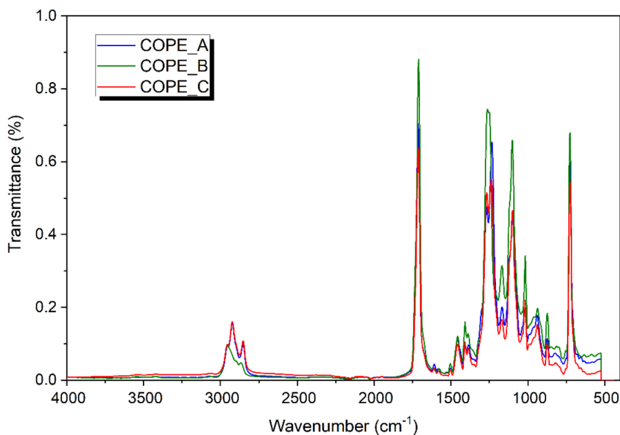
Figure 2. The comparison of FTIR spectra of studied HMAs.
