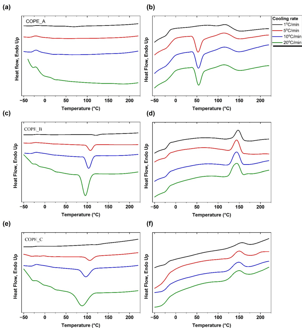
Figure 5. (a) DSC cooling scans of COPE_A; (b) second DSC heating scans of COPE_A; (c) DSC cooling scans of COPE_B; (d) second DSC heating scans of COPE_B; (e) DSC cooling scans of COPE_C; (f) second DSC heating scans of COPE_C. Four different cooling rates were applied and one constant heating rate (10°C/min.).
