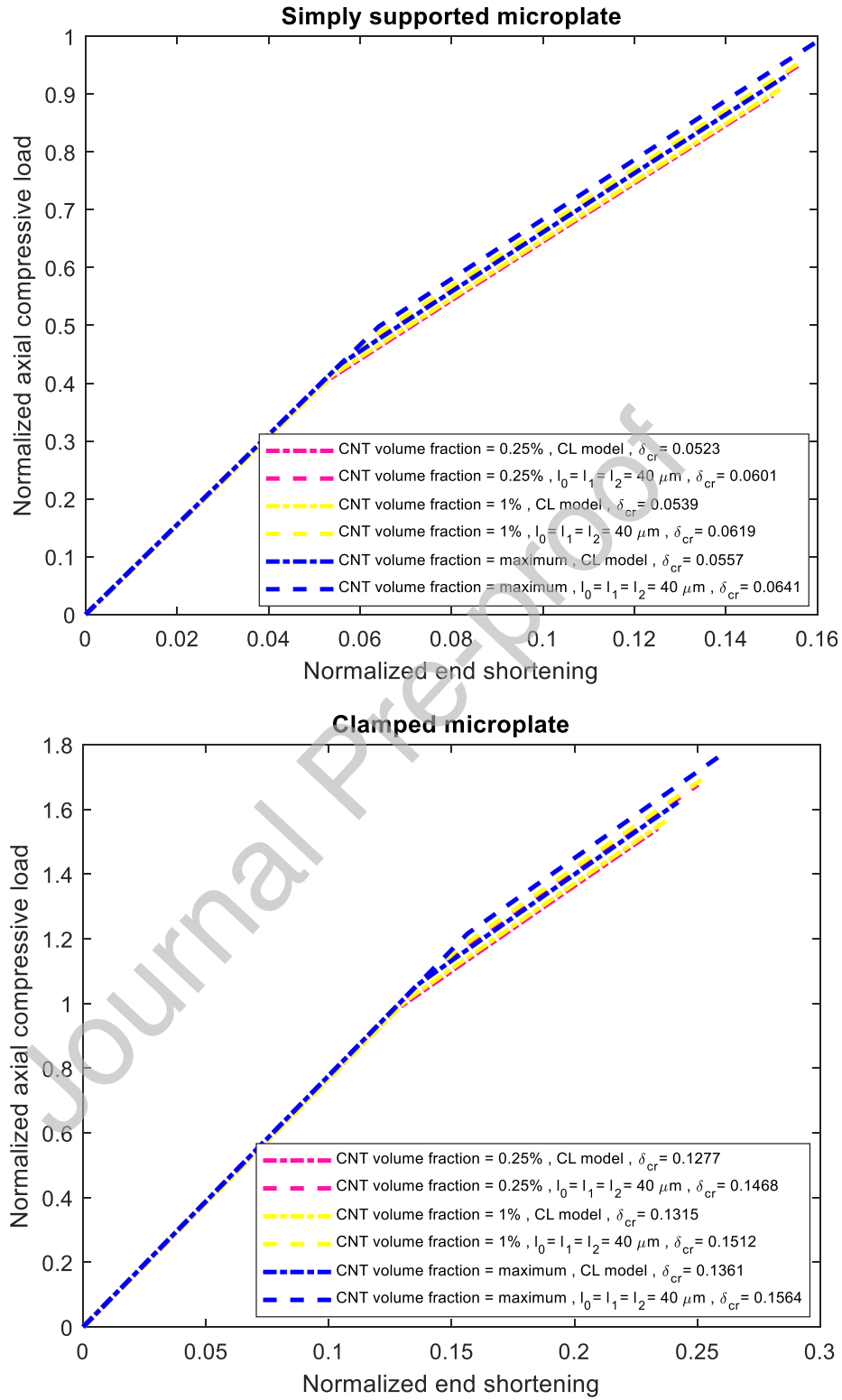
Fig. 15. CL-based and MSGT-based load-shortening nonlinear equilibrium graphs allocated to different values of CNT volume fraction ( l_T = 0.39 \text{ nm} , l_S = 43.4 \text{ GPa} , V_{GF} = 50\% )
