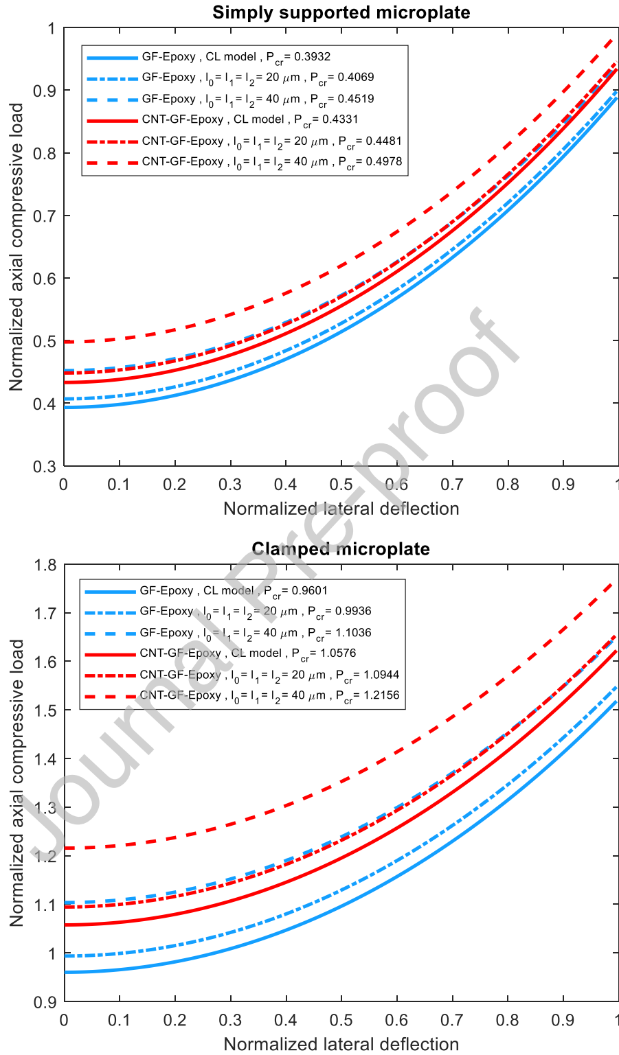
Fig. 10. CL-based and MSGT-based load-deflection nonlinear equilibrium graphs allocated to different values of small scale parameters ( l_T = 0.39 \text{ nm} , l_S = 43.4 \text{ GPa} , V_{CNT} = \text{maximum} , V_{GF} = 50\% )
