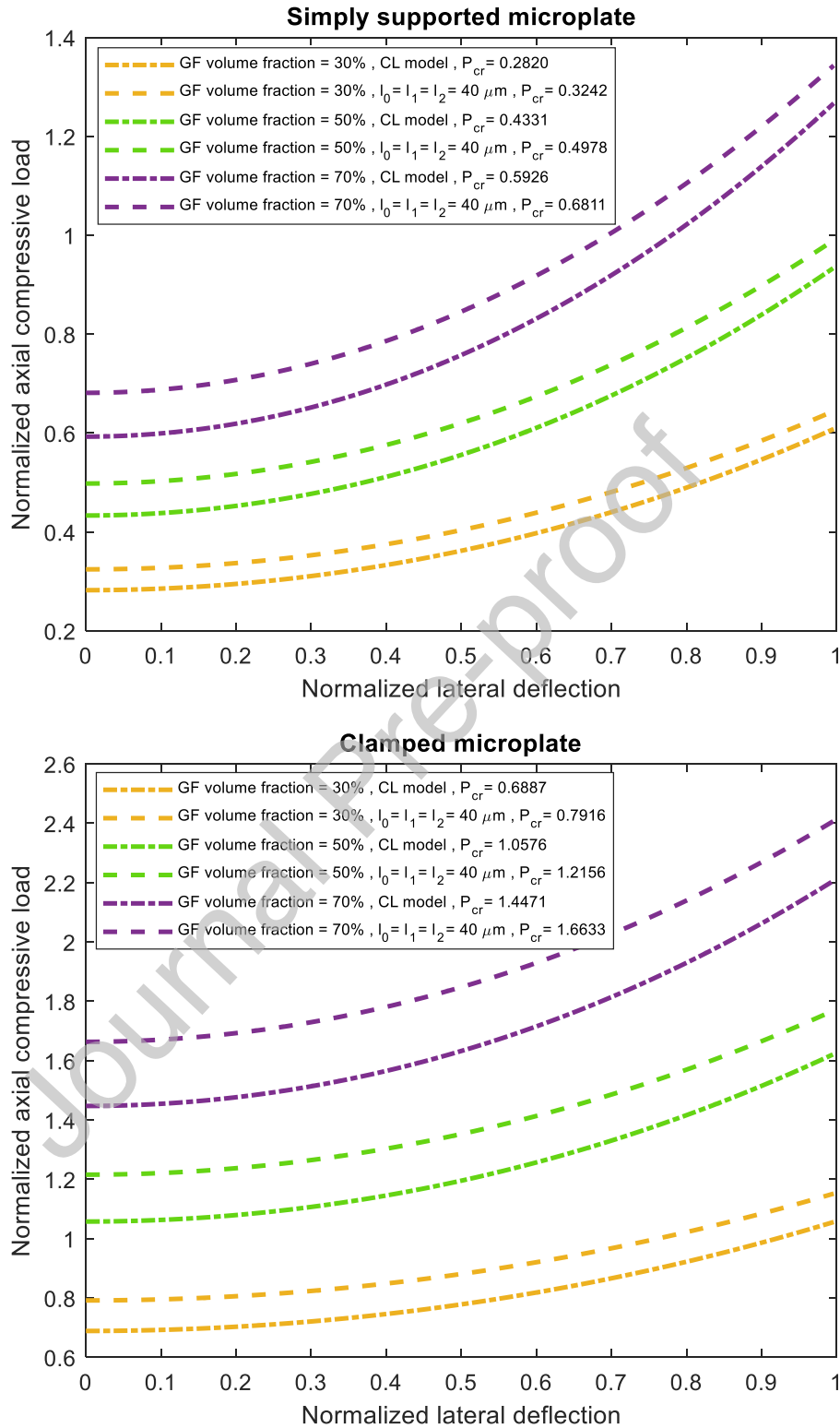
Fig. 12. CL-based and MSGT-based load-deflection nonlinear equilibrium graphs allocated to different values of GF volume fraction ( l_T = 0.39 \text{ nm} , l_S = 43.4 \text{ GPa} , V_{CNT} = \text{maximum} )
