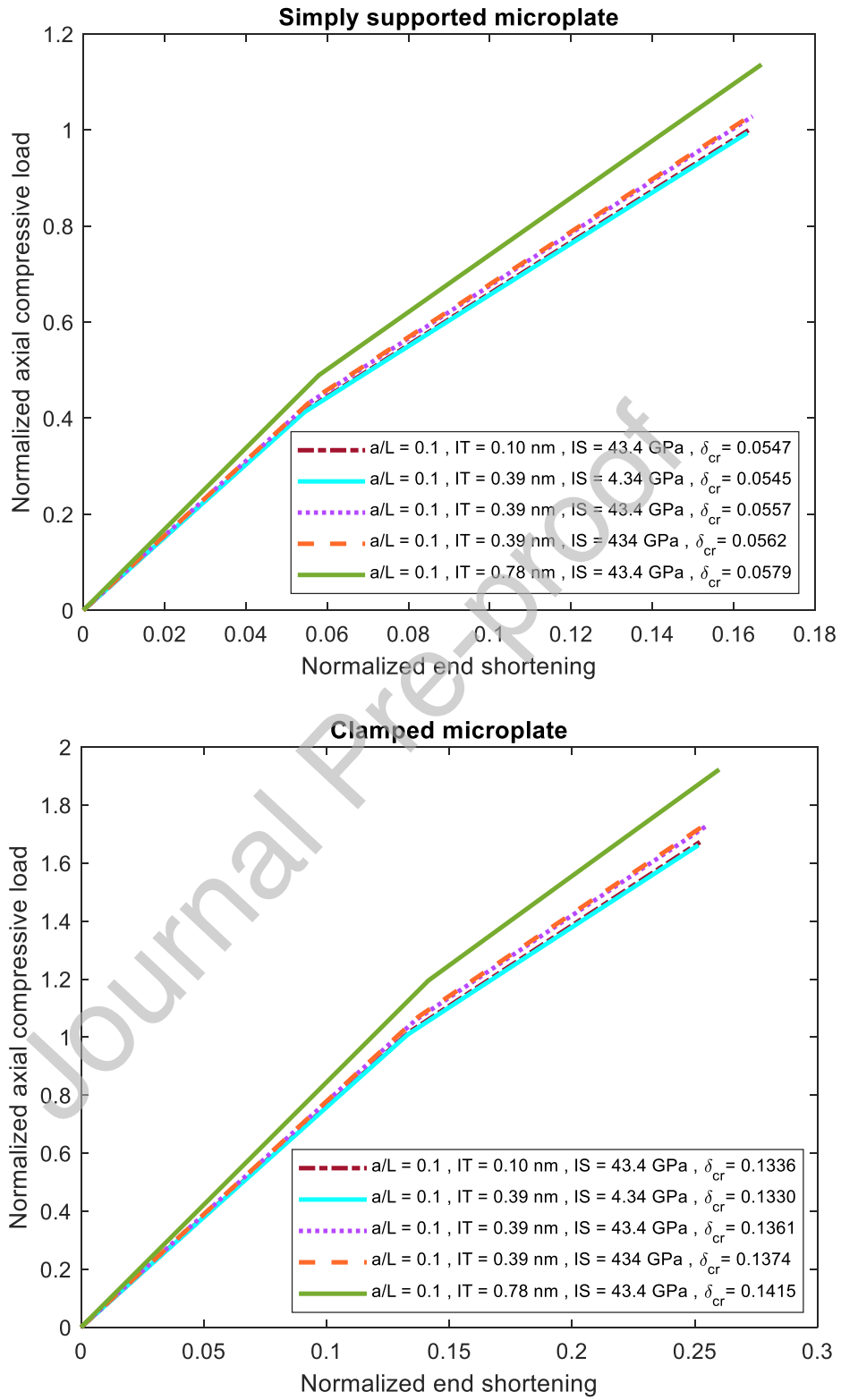
Fig. 23. MSGT-based load-shortening nonlinear equilibrium graphs allocated to the microplate having a central square cutout ( l_0 = l_1 = l_2 = 40 \mu m , V_{CNT} = \text{maximum} , V_{GF} = 50\% )
